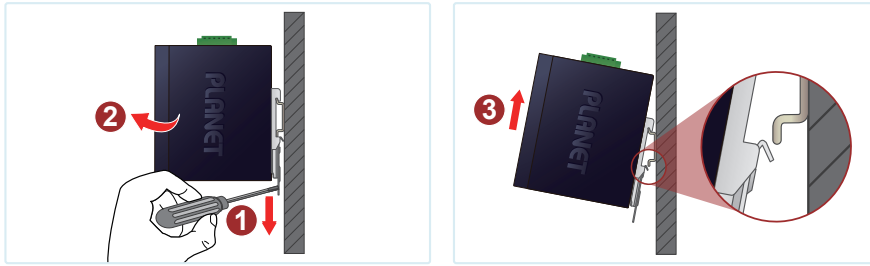
IFGS-624PTF DIN-rail Mounting Installation
