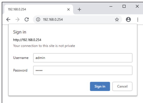
Figure 5-2: Login Screen
