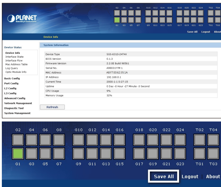
Figure 5-4: Save Configuration
