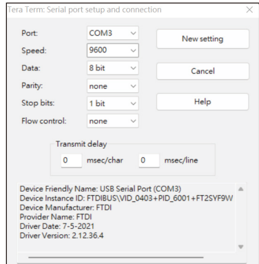
Figure 4-2: Tera Term COM Port Configuration
