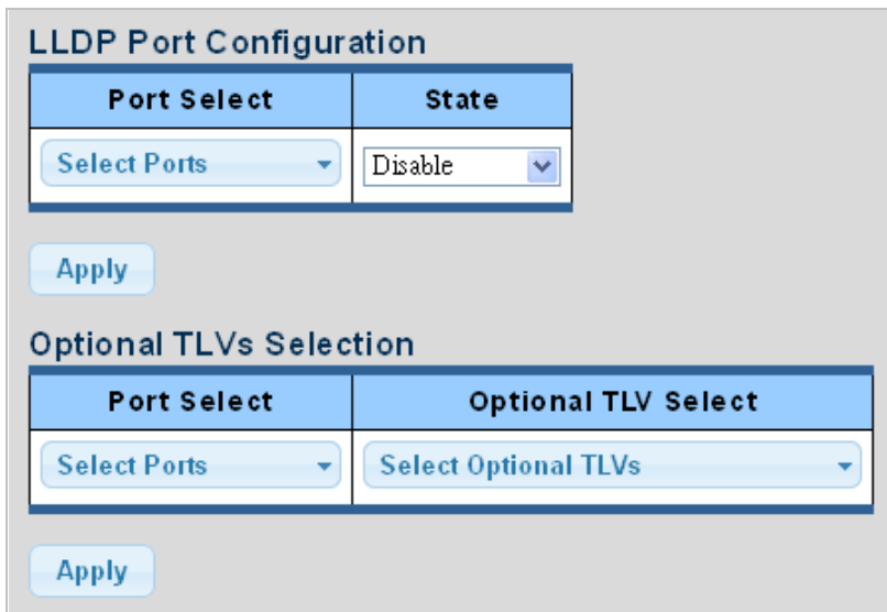
Figure 4-3-114 LLDP Port Configuration and Optional TLVs Selection Page Screenshot
