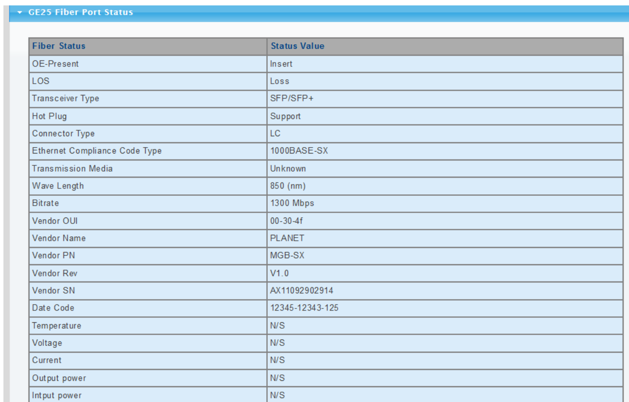
Figure 4-3-21 Fiber Port Status Page Screenshot
