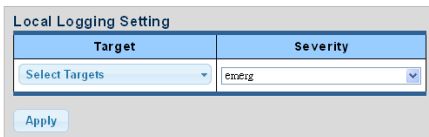
Figure 4-2-14 Local Log Target Setting Page Screenshot
