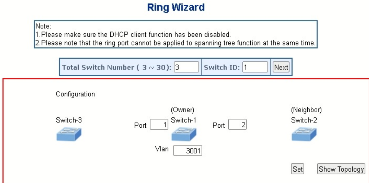
Figure 4-6-1 Ring Wizard page screenshot
