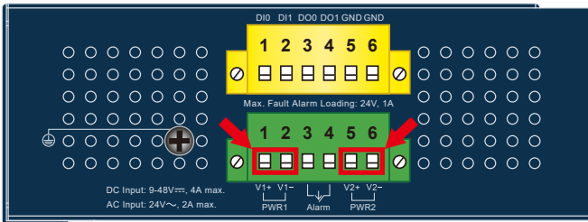
Figure 3-1: IGS-6325-5X1T Upper Panel
