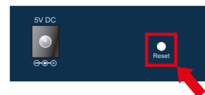
Figure 7-1: ICS-110/ICS-115A Hardware-based Reset Button
