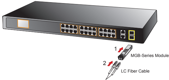
Figure 3-4: Plugging in the SFP Transceiver
