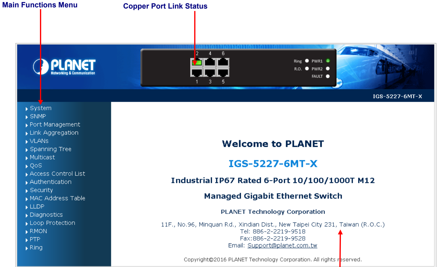
Figure 4-1-4: Main Page
