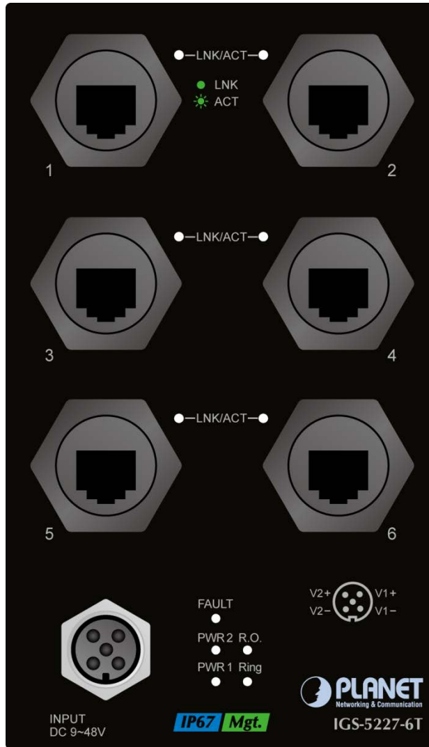
Figure 2-1: IGS-5227-6T Switch Front Panel
