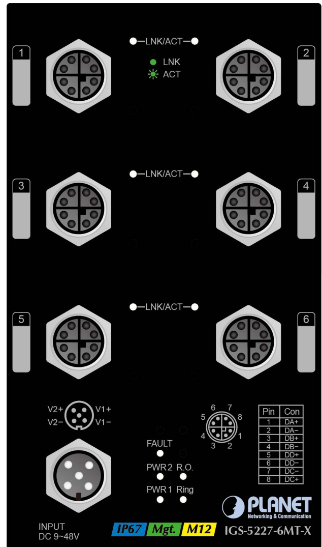
Figure 2-3 IGS-5227-6MT-X Switch Front Panel
