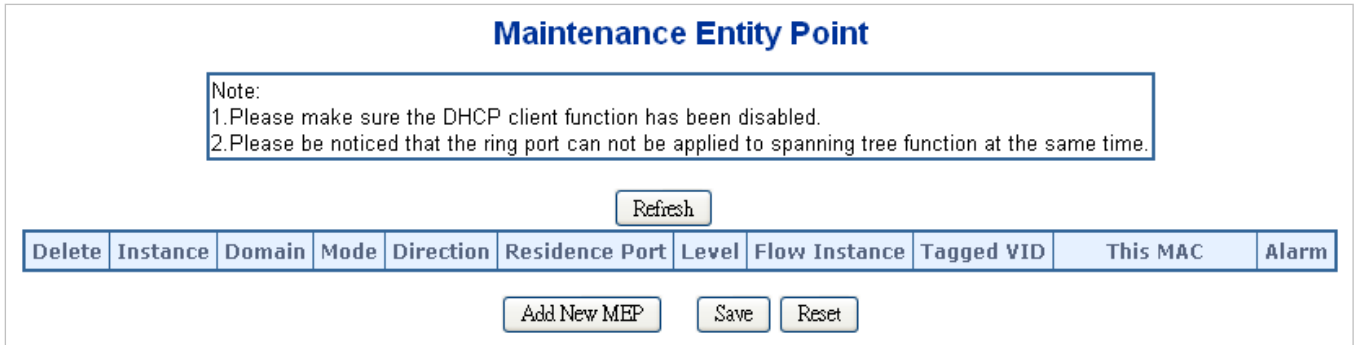
Figure 4-19-1: MEP Configuration Screenshot
