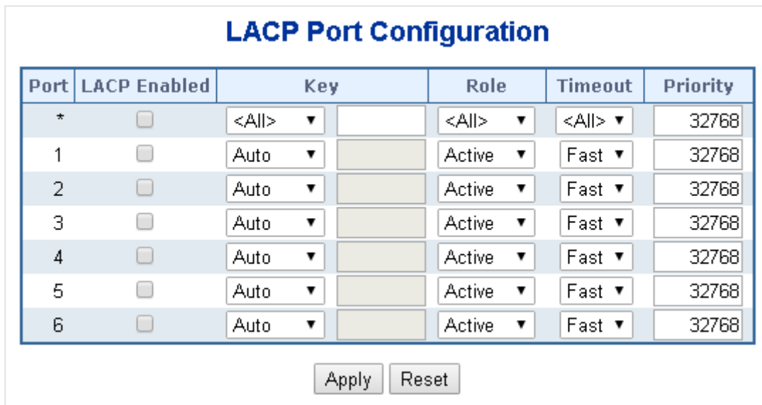
Figure 4-5-4 : LACP Port Configuration Screenshot
