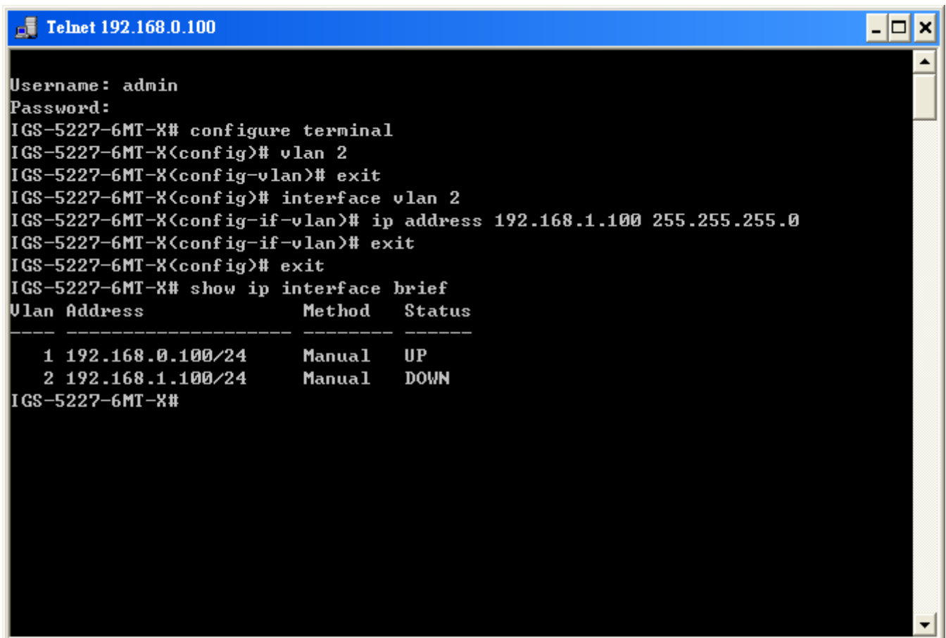
Figure 3-1: Remote Telnet Interface Main Screen of Industrial Managed Switch
