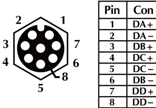
8-pin M12 A-coded Female 10/100/1000T Connector Pin Assignment
