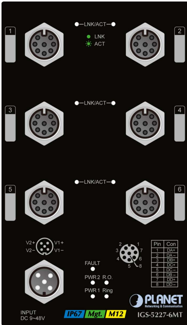
Figure 2-2 IGS-5227-6MT Switch Front Panel
