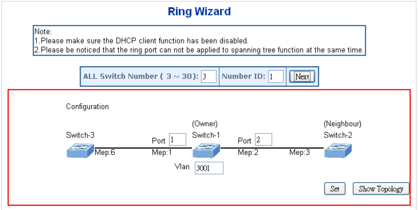
Figure 4-19-5: Ring Wizard Screenshot
