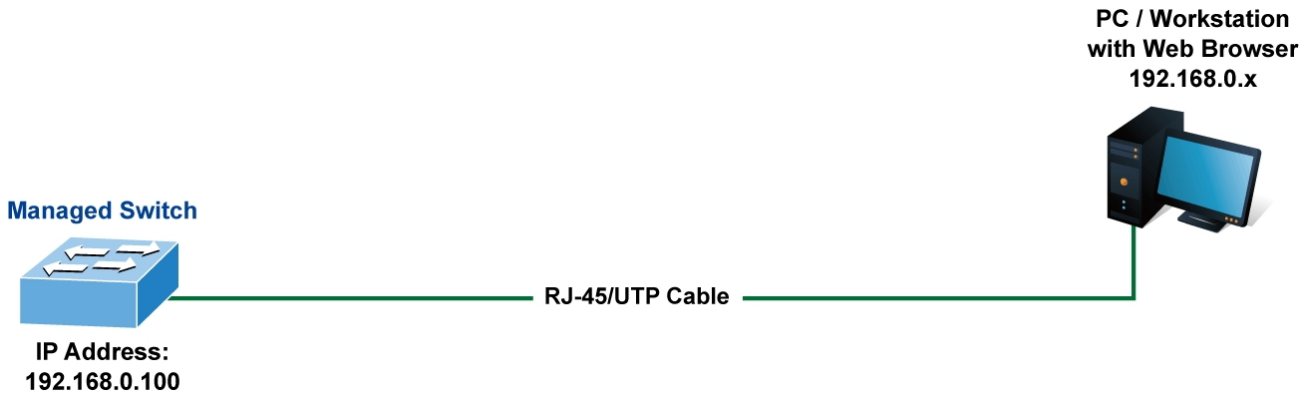
Figure 3-2: Web Management
