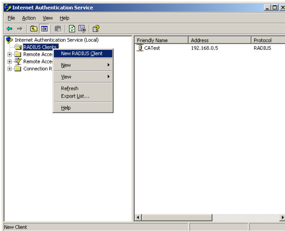
Figure 4-11-12: Windows Server – Add New RADIUS Client Setting
