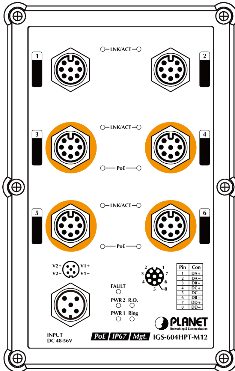
Figure 2-1: IGS-604HPT-M12 Switch Front Panel
