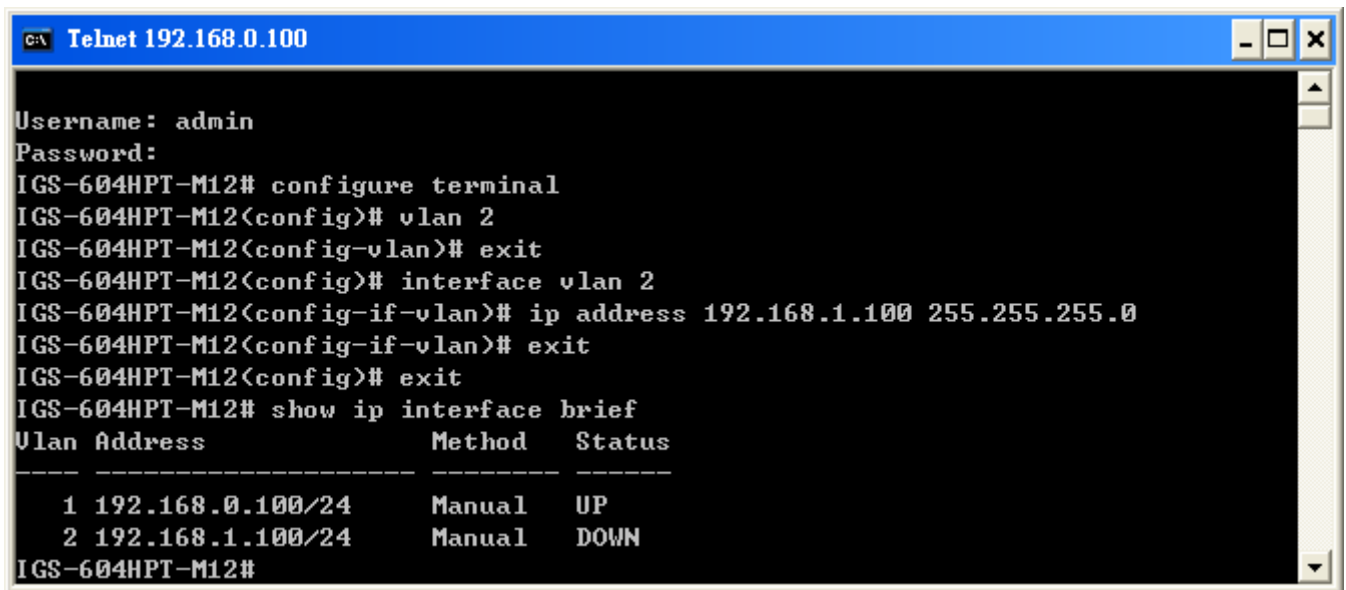
Figure 3-1: Remote Telnet Interface Main Screen of Industrial Managed Switch
