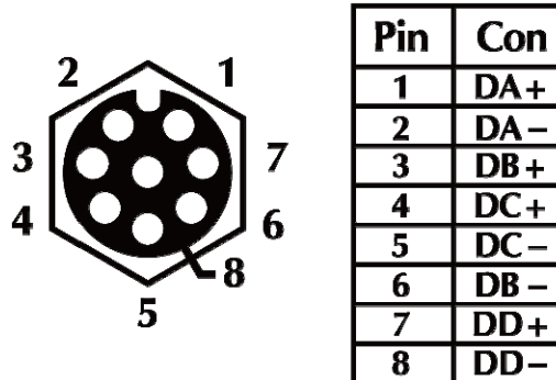
8-pin M12 Female 10/100/1000T Connector Pin Assignment
