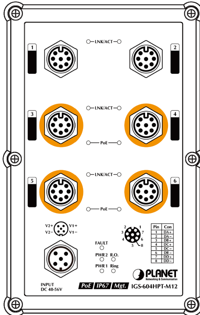
Figure 2-2: IGS-604HPT-M12 LED on Front Panel
