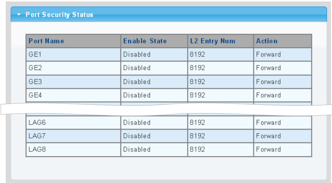
Figure 4-13-31: Port Security Status Page Screenshot
