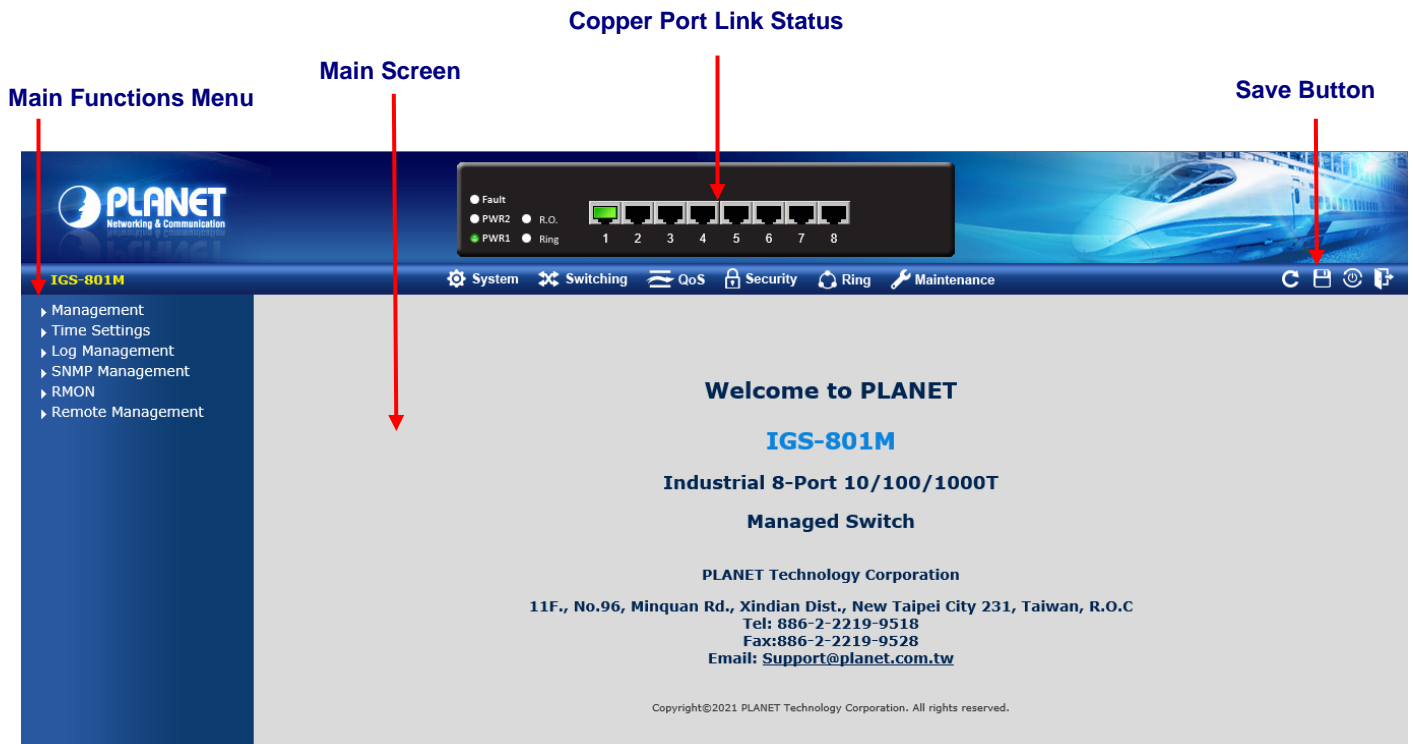
Figure 4-1-4: Web Main Page
