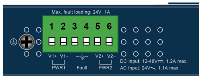
Figure 2-1-4: IGS-801M Top View
