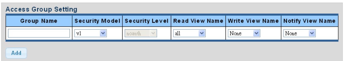
Figure 4-2-25: SNMPv3 Access Group Setting Page Screenshot
