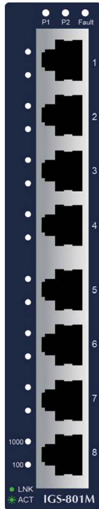
Figure 2-1-3: IGS-801M LED Panel
