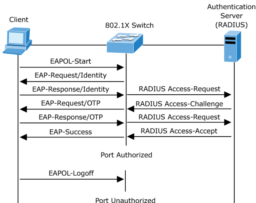
Figure: EAP Message Exchange
